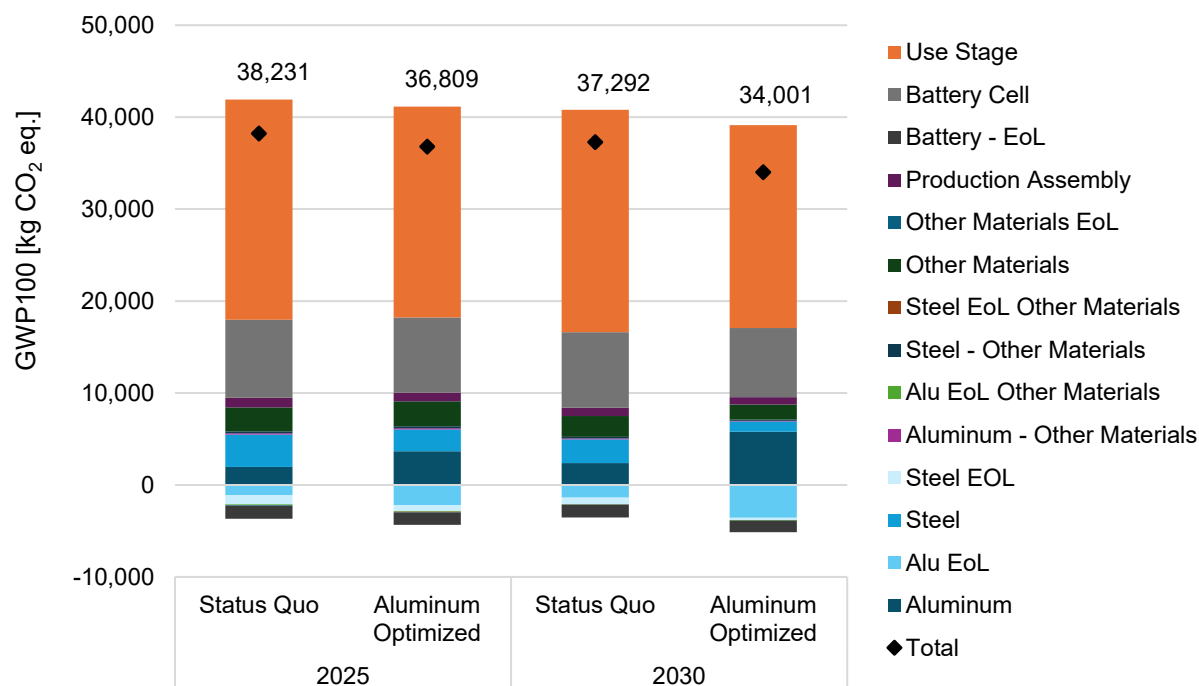
Figure ES 2: Contributions of materials and life cycle stages to GWP100 per Family Crossover with a lifetime mileage of 200,000 miles
