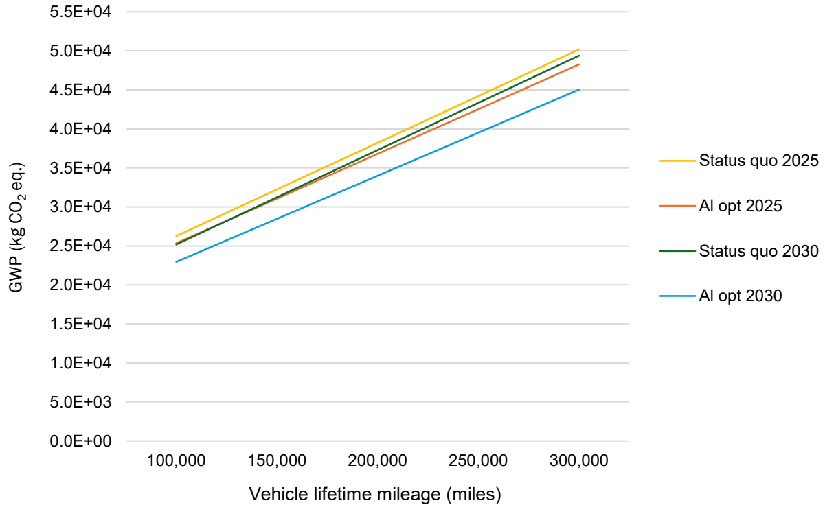
Figure 4-12: Sensitivity of lifetime GWP100 to Family Crossover lifetime mileage
