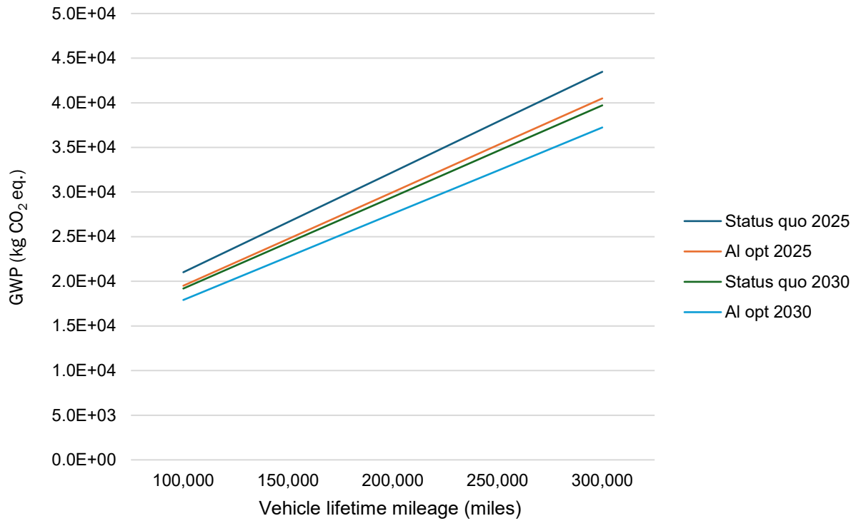
Figure 4-11: Sensitivity of lifetime GWP100 to City Vehicle lifetime mileage
